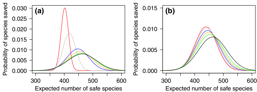
Figure 5. The change in probability distributions of the expected number of species safe from extinction (a) when thresholds of managers' levels of unacceptable risk are applied, below which species projects are excluded (black, no threshold; green, 30% threshold; orange, 50%; blue, 70%; grey, 90%; and red, 100%) and (b) for a variance-discounting approach with increasing \alpha representing higher levels of unacceptable risk and corresponding aversion to the probability of management failure (black, zero alpha [no risk aversion]; green, 0.3; orange, 0.5; blue, 0.7; grey, 0.9; red, 1.0).
